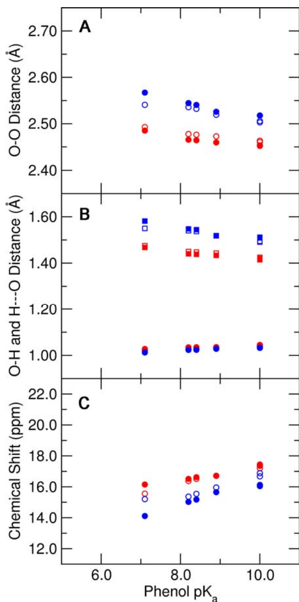
Figure S2: Comparison of the results obtained from QM/MM geometry optimizations with two different solvent configurations obtained after 500 ps (open symbols) and 1 ns (filled symbols) of solvent molecular dynamics. The following quantities are depicted as functions of the solution pK a of the substituted phenolate: (A) the hydrogen bond O–O distances, (B) the hydrogen bond O–H distances (circles) and H---O distances (squares), and (C) the calculated NMR chemical shifts. The Tyr16-phenolate hydrogen bond is shown in red, while the Asp103-phenolate hydrogen bond is shown in blue. The ligands in these calculations were phenol, 4-fluorophenol, 3,5-difluorophenol, 3,4,5-trifluorophenol, 4-trifluoromethylphenol, and 4-nitrophenol. All calculations included Tyr16, Asp103, Asp40Asn, and the phenolate in the QM region.
